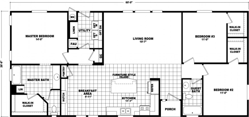
MODEL: MR-28603B APPROXIMATELY 1600 SQ. FT. TOTAL APPROXIMATELY 1579 SQ. FT. LIVABLE 3 BEDROOM, 2 BATH
