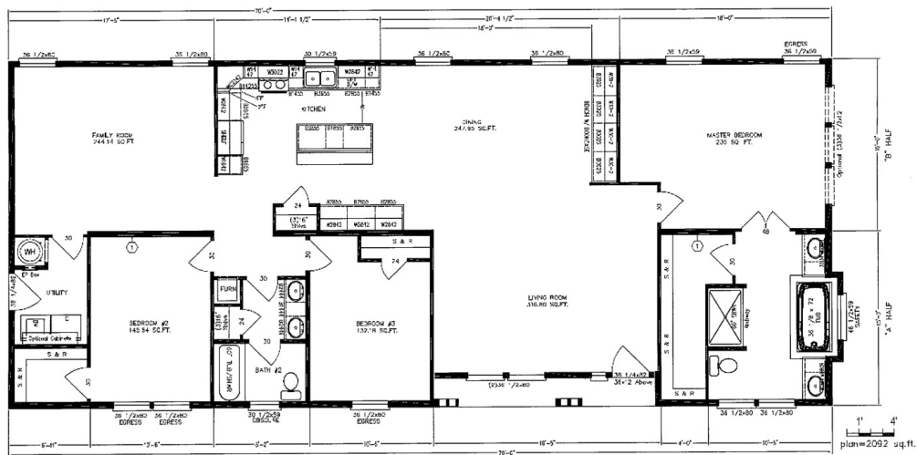
ROCK CREEK HD30703P 2060 Sq.ft.
